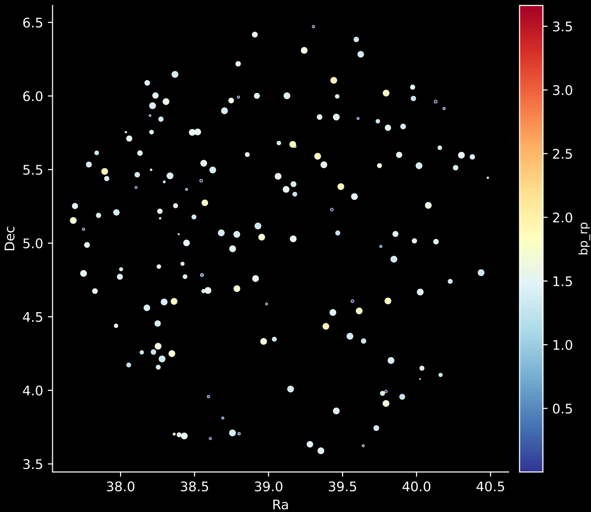
APOGEE DR17 Field: [045-12] Stars: 156
