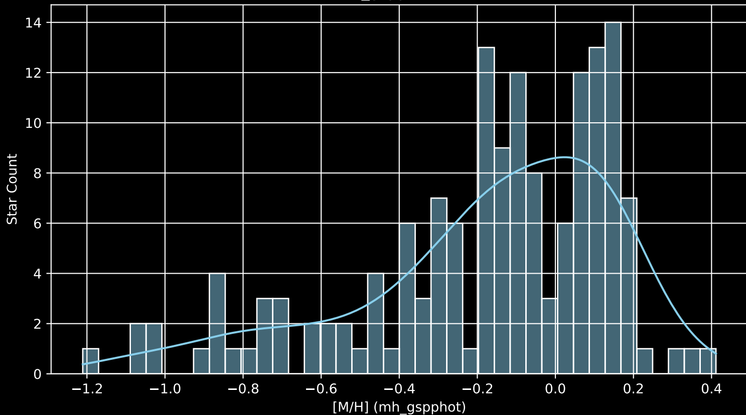
APOGEE DR17 Field: [045-12 [M/H] (mh_gspphot) (n= 154)
