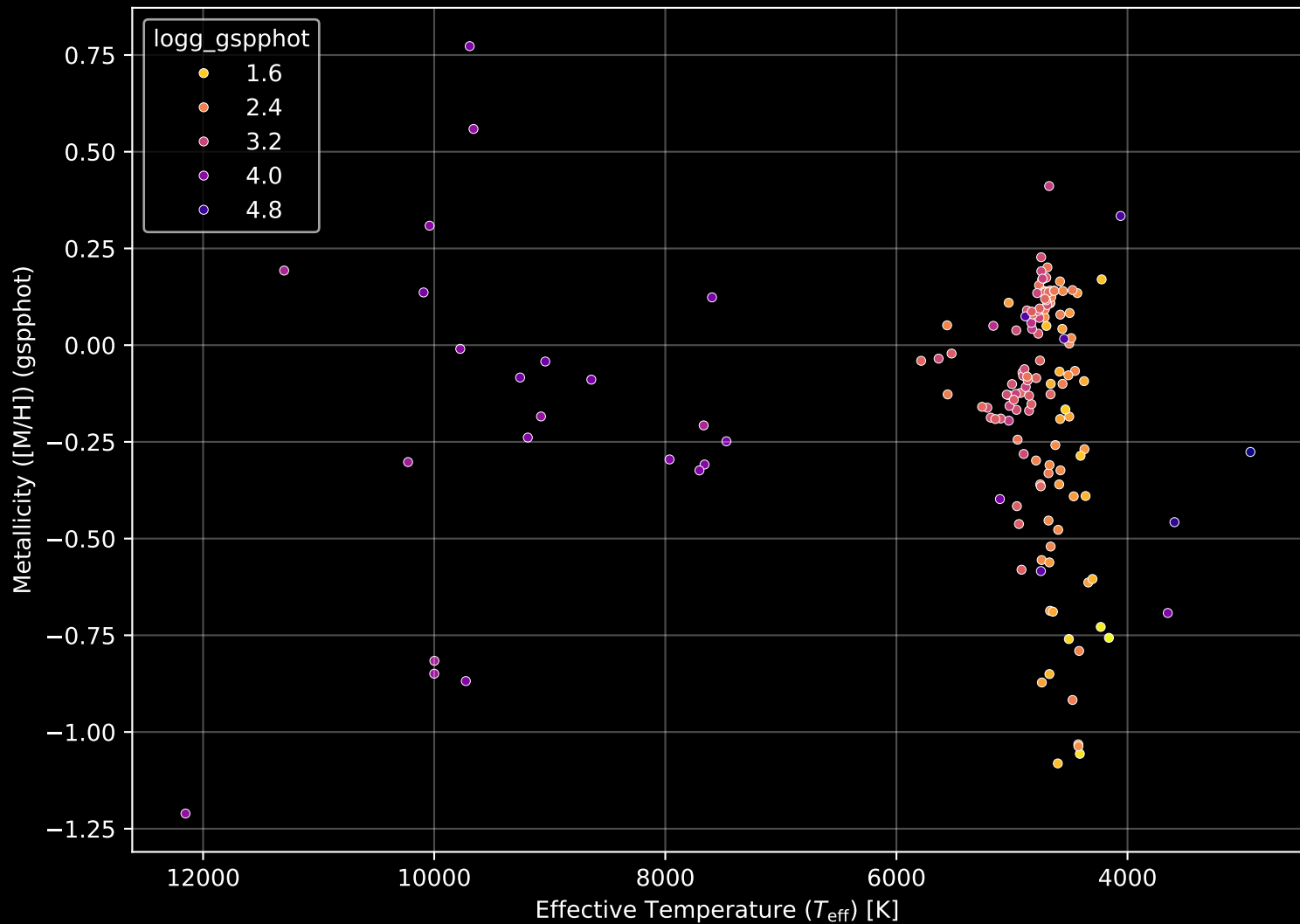
APOGEE DR17 Field: [045-12] Stellar Population Parameters (n= 156)
