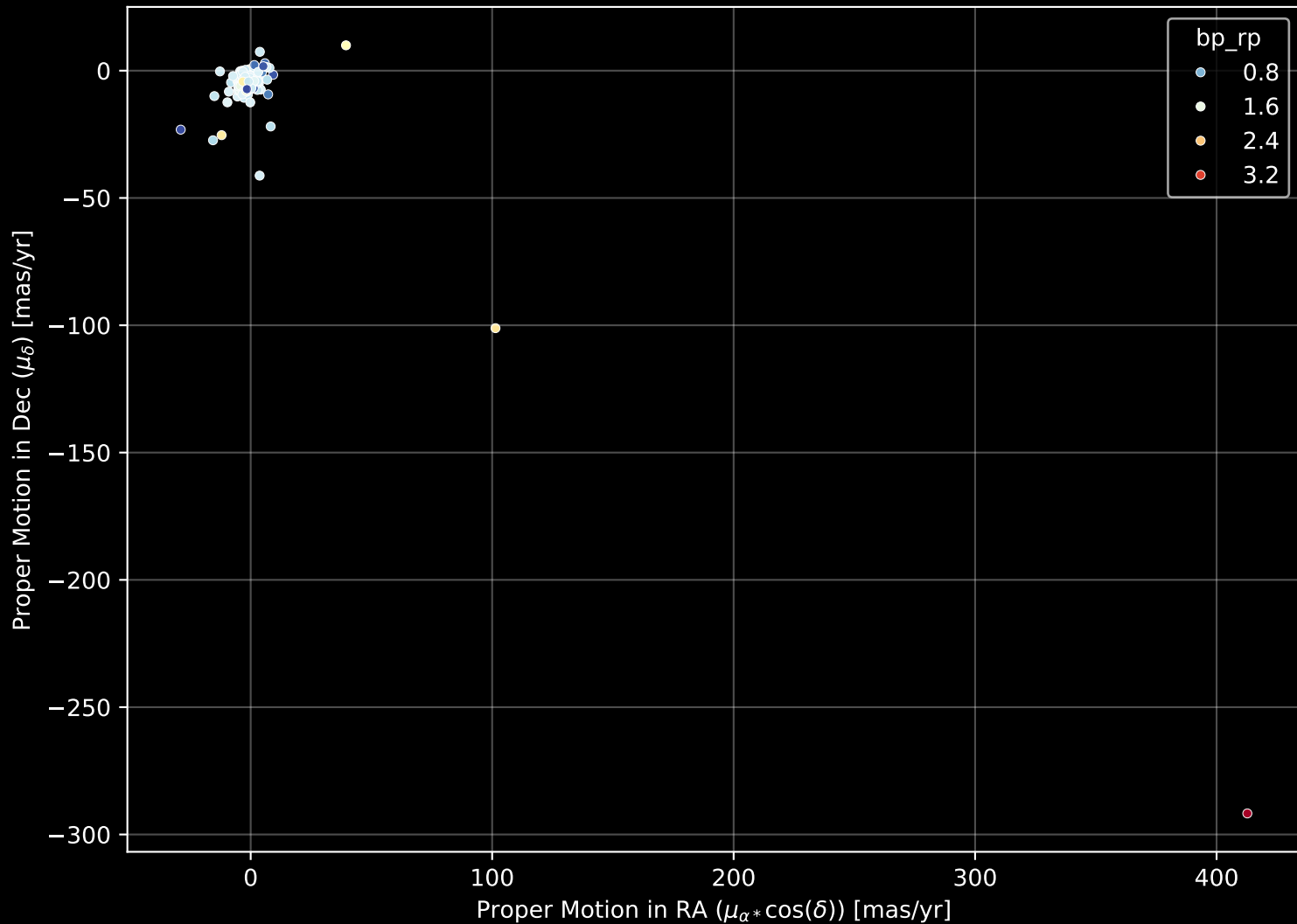
APOGEE DR17 Field: [045-12] Proper Motion Diagram (n= 156)
