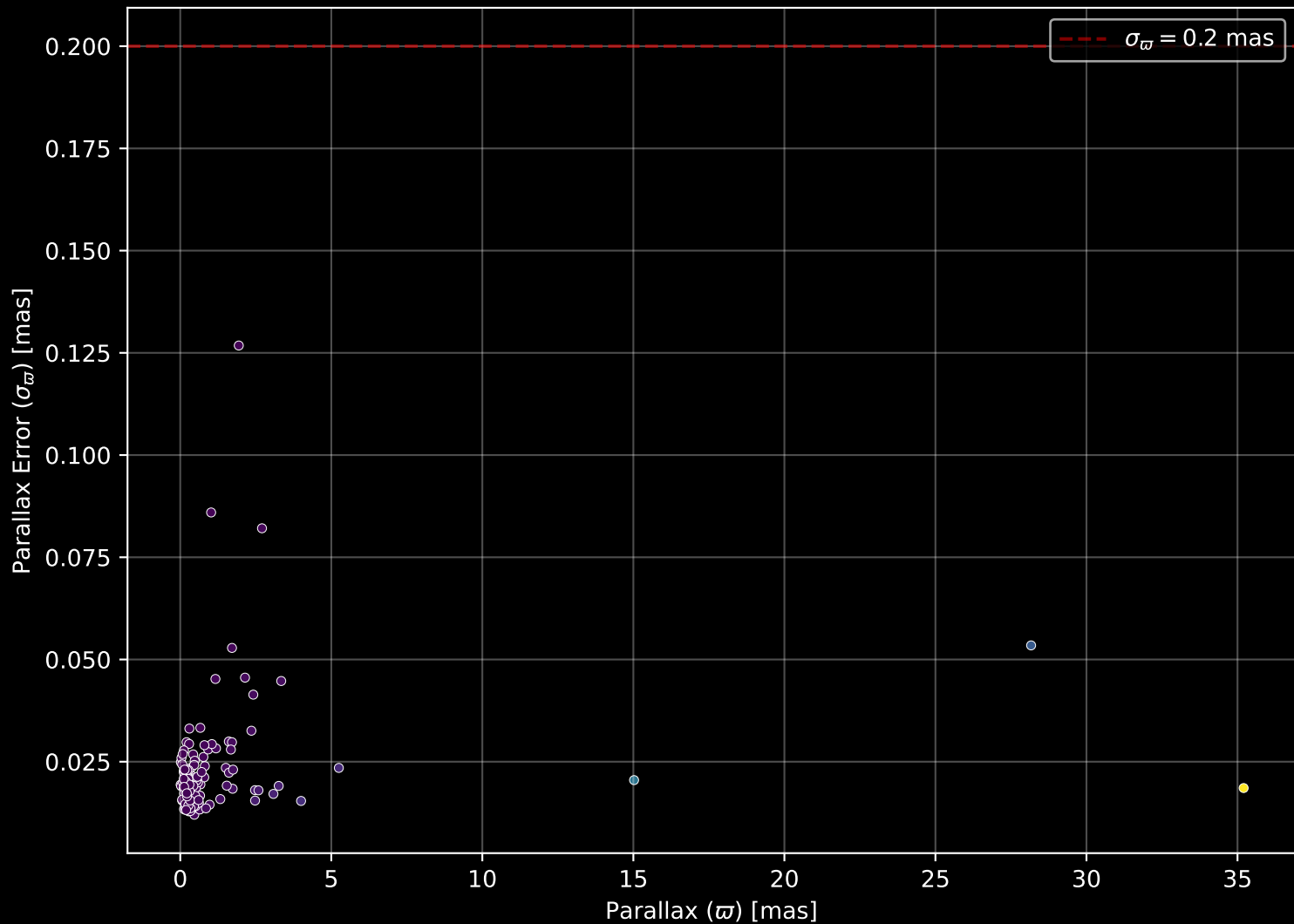
APOGEE DR17 Field: [045-12] Parallax Quality (n= 156)
