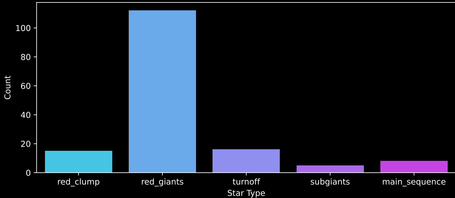
APOGEE DR17 Field: [045-12] Count plot of Star Type
