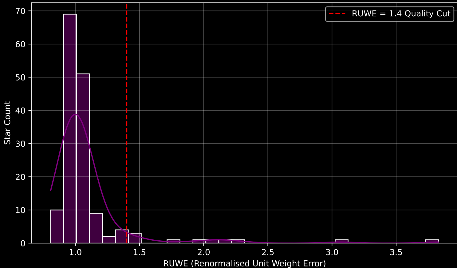
GAPOGEE DR17 Field [045-12] RUWE Distribution (n= 155)
